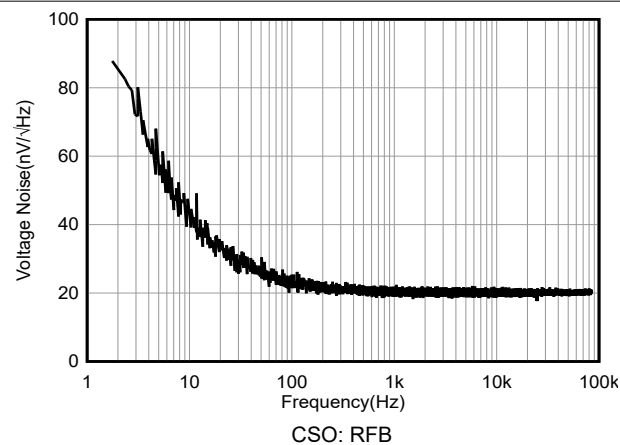
Figure 5-12. Voltage Noise
