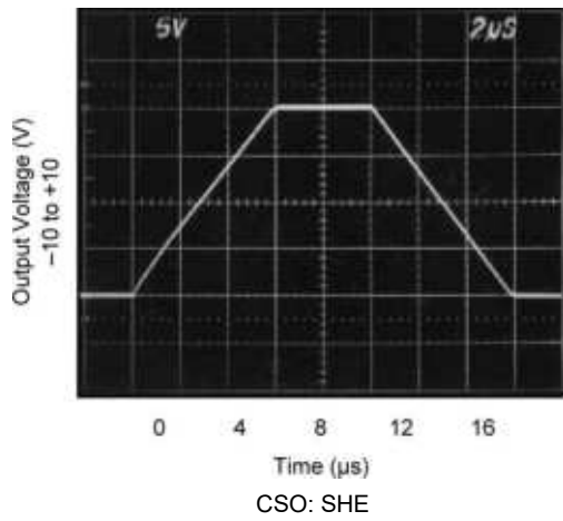
Figure 5-1. Step Response
