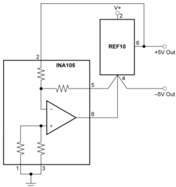
Figure 7-21. \pm 5V Precision Voltage Reference
