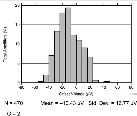
Figure 7-4. Typical Distribution of Offset Voltage (RTO)
