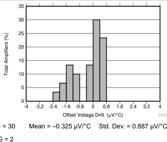
Figure 7-6. Typical Distribution of Offset Voltage Drift (RTO)
