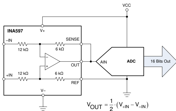
Differential Input Data Acquisition
