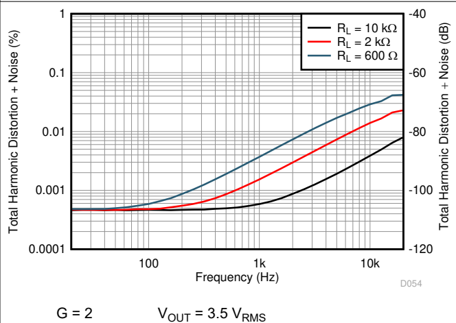
Figure 7-54. THD+N vs Frequency
