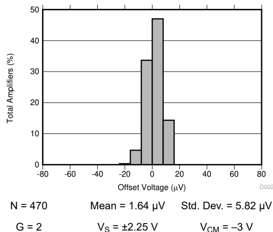
Figure 7-2. Typical Distribution of Offset Voltage (RTO)
