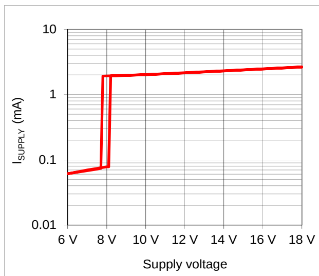
Figure 5: Supply Current vs. Supply Voltage
