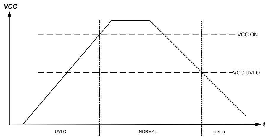
Figure 3: Vcc UVLO
