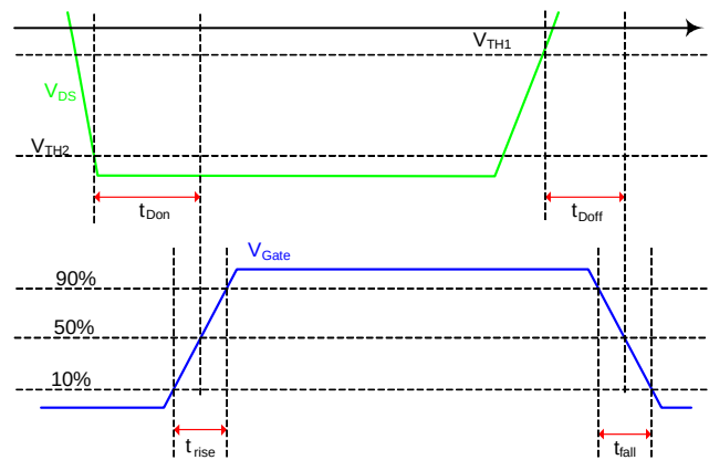
Figure 4: Timing waveform
