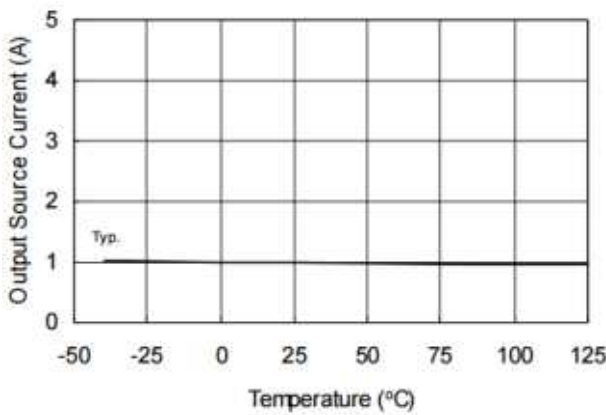
Figure 19A. Output Source Current vs. Temperature
