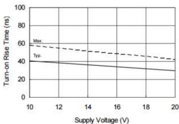
Figure 4B. Turn-on Rise Time vs. Supply Voltage
