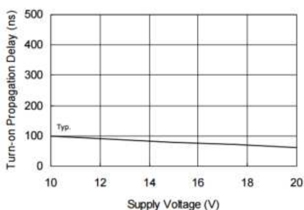
Figure 2B. Turn-on Propagation Delay vs. Supply Voltage
