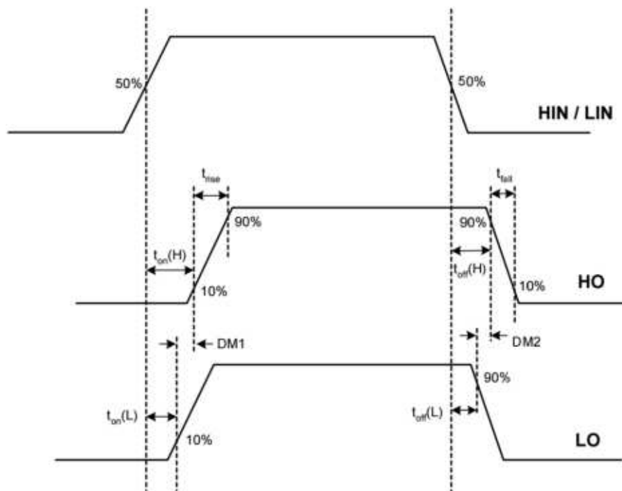
Figure 1. Timing Diagram
