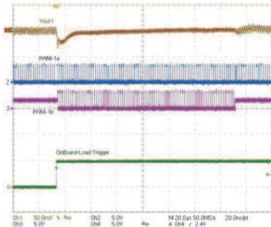
Figure 29: loop1 going from 1 \Phi to 2 \Phi operation due to a heavy load transient which causes Vout drop, 1 \Phi operation is resumed with a delay after Vout1 recovers.
