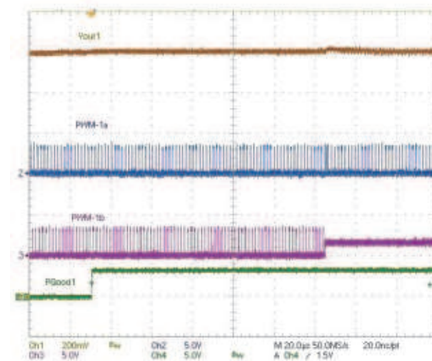
Figure 28: Phase Shed 2 \Phi 1 \Phi at startup
