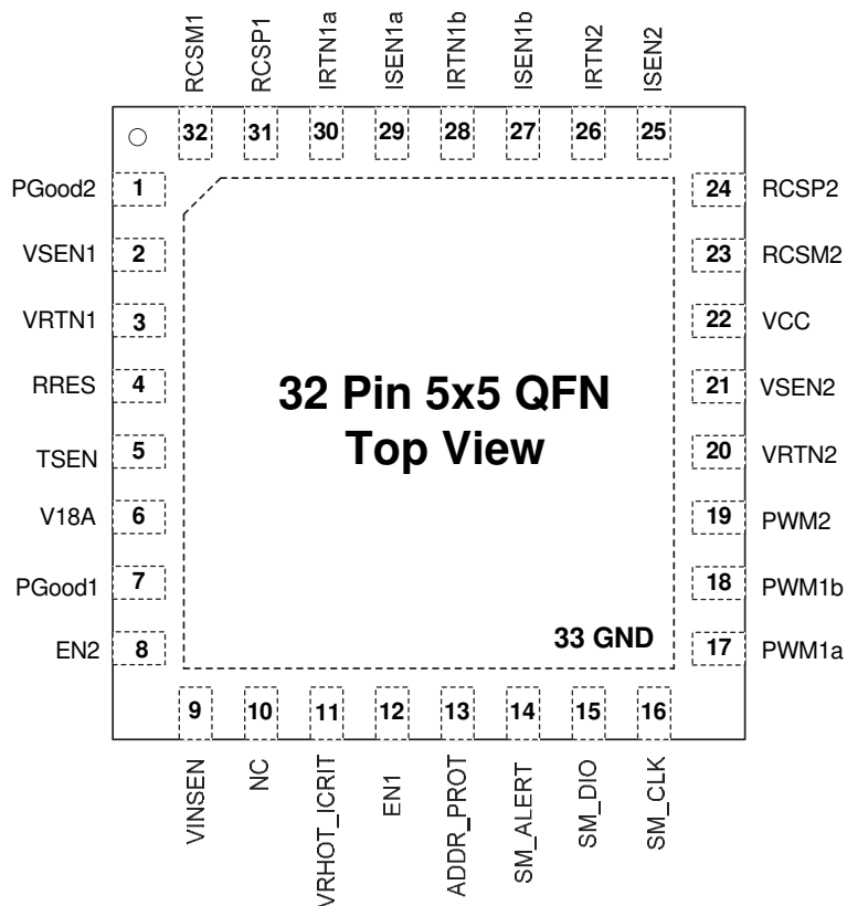
Figure 3: IR36021 Package Bottom View 5mm X5mm QFN
