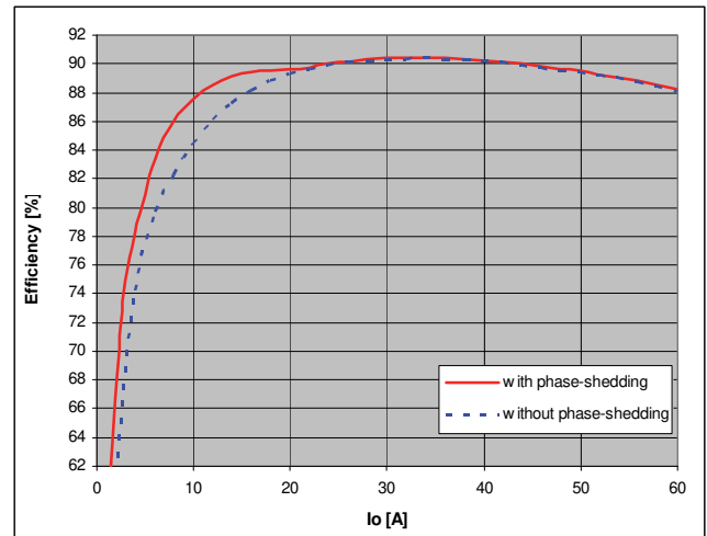
Figure 31: Typical Efficiency with phase-shedding for loop1, Vo1=1.2V, 600kHz/phase, 2 x IR3550 used as power-stages
