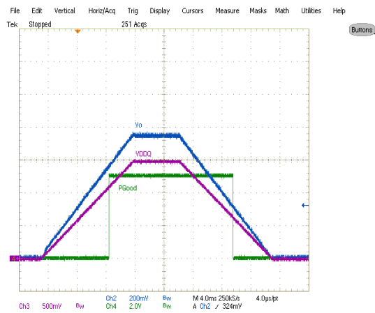
Fig. 22: Tracking 8A, sourcing current, Ch_2:V_{out} , Ch_3:V_{DDQ} , Ch_4:P_{Good}
