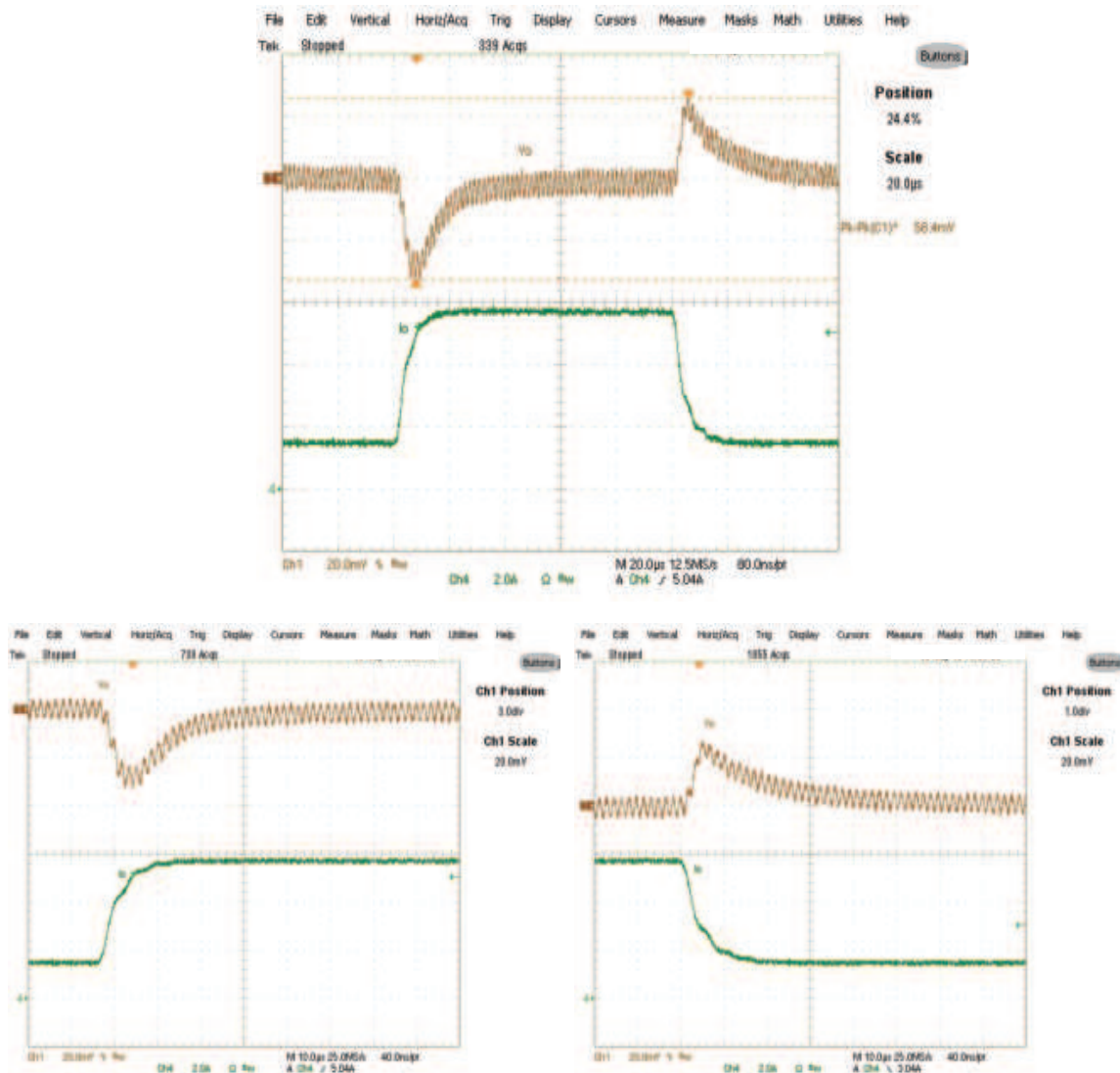
Fig. 28: Transient Response 1.4A(10%)-5.6A(40%) load (0.5A/us) Ch_1:V_{out} , Ch_4:I_o
