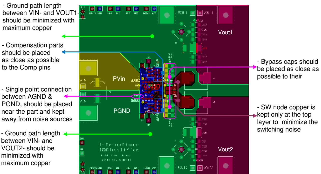
Figure 42a: IRDC3892 Demo board Layout Considerations – Top Layer
