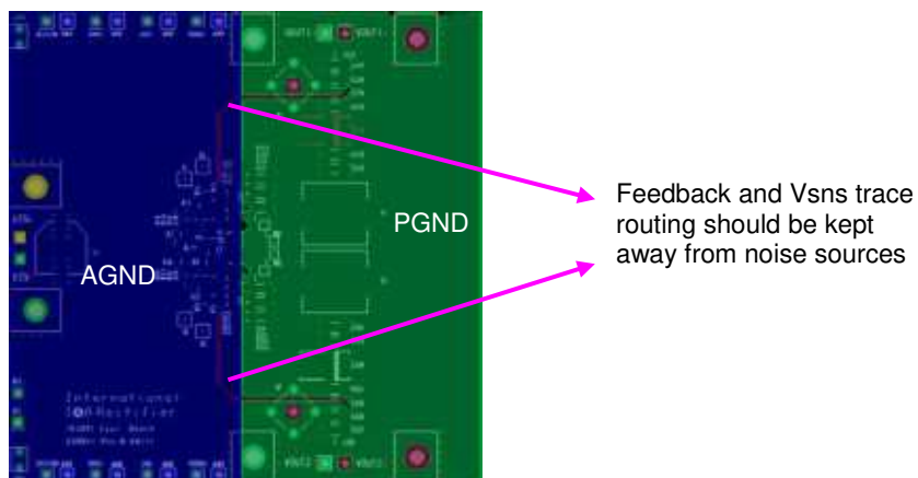
Figure 42c: IRDC3892 Demo board Layout Considerations – Mid Layer 1
