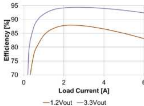
Figure 2: Efficiency [Vin=12V, Fsw=600kHz]
