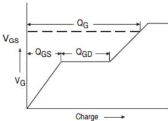
Fig 13a. Basic Gate Charge Waveform
