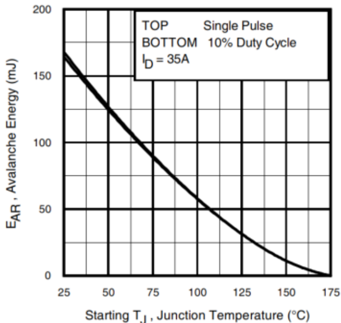
Fig 16. Maximum Avalanche Energy vs. Temperature
