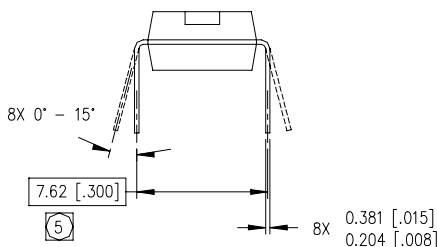
8-Lead PDIP
