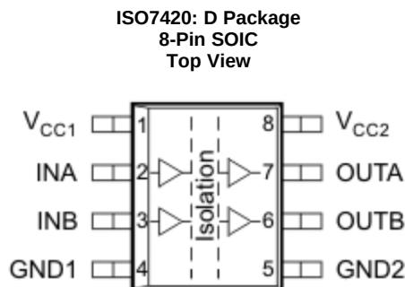
Pin Functions
