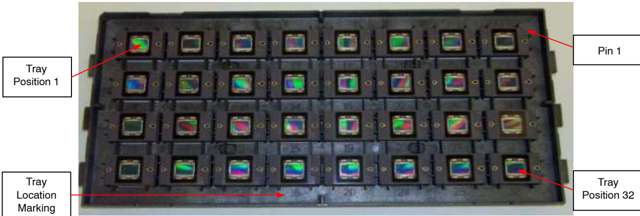
Figure 35. Tray Pin-Down View
