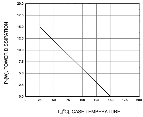
Figure 8. Power Derating
