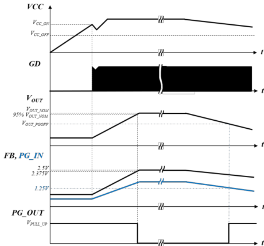
Figure 17. PGOOD timing
