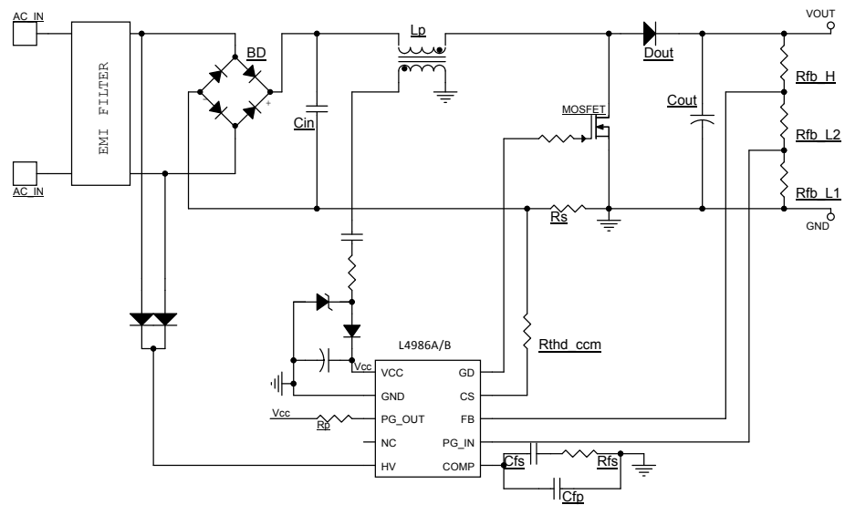
Figure 2. Typical application
