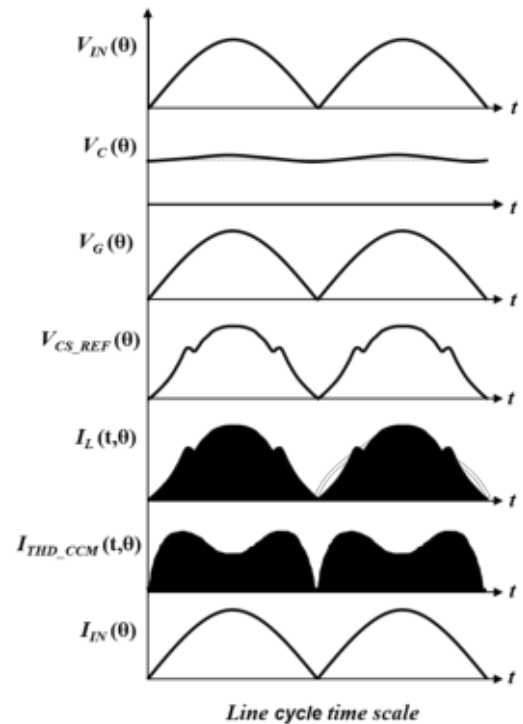
Figure 6. Right key waveforms of the circuit in figure 4 – Line cycle time scale
