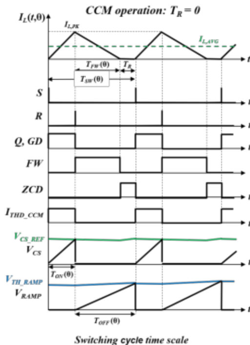
Figure 5. Left key waveforms of the circuit in figure 4 – Switching cycle time scale
