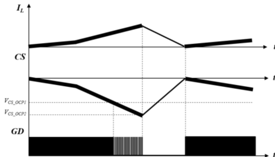
Figure 19. OCP2 timing
