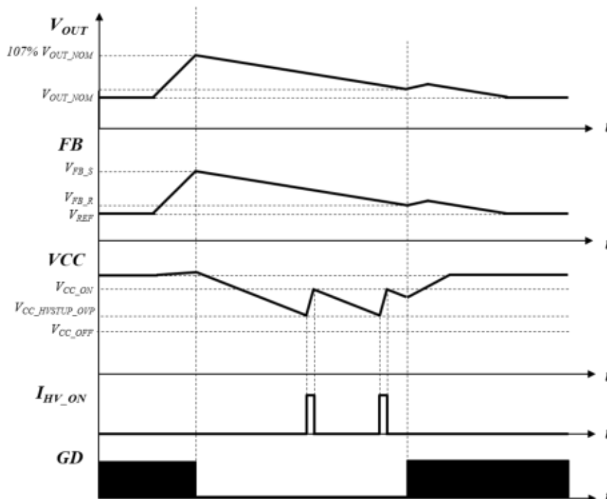
Figure 18. OVP timing
