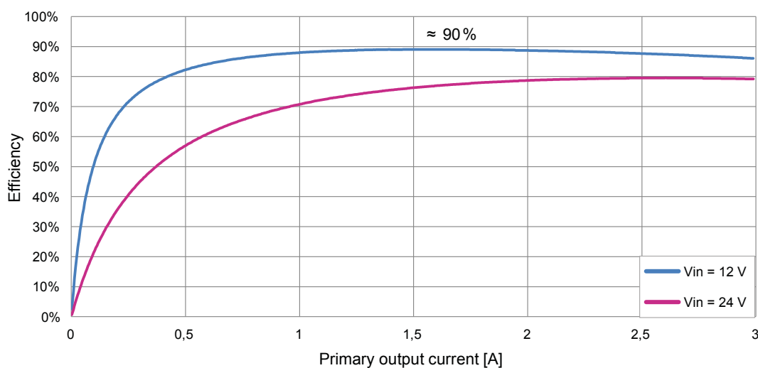
Figure 23. Primary output efficiency ( V_{OUT\_prim} = 5\text{ V} , f_{SW} = 400\text{ kHz} , secondary isolated output not loaded)
