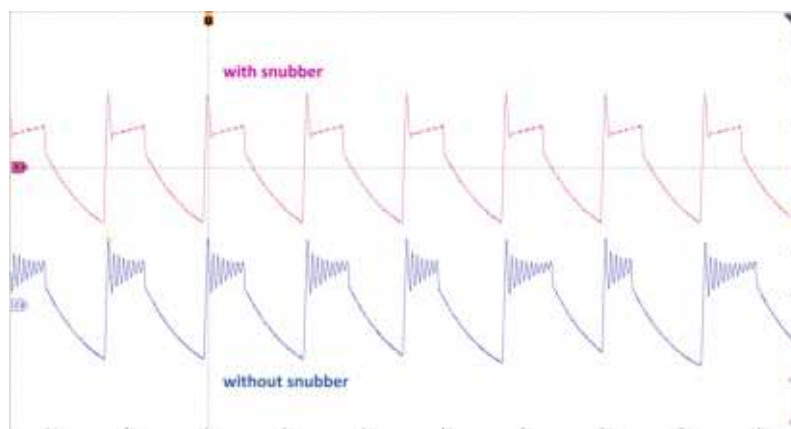
Figure 47. Filtering effect of the snubber network
