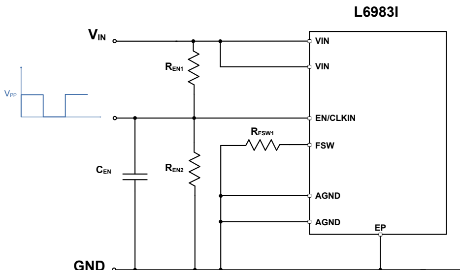
Figure 42. External synchronization (AC coupling)
