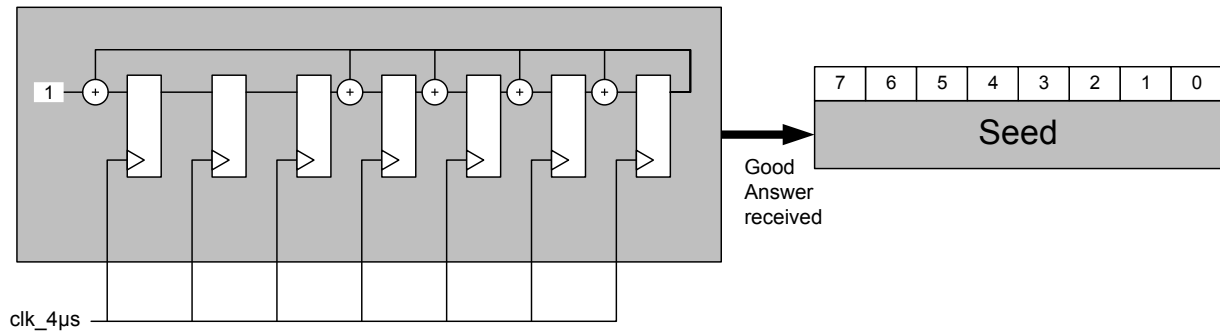
Figure 57. Seed generation algorithm block diagram
