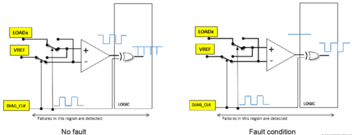
Figure 69. Diagnostic analog self test basic implementation
