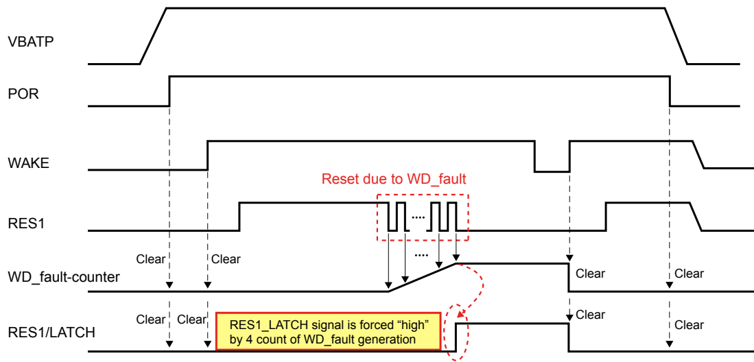
Figure 49. Reset-Latch timing diagram
