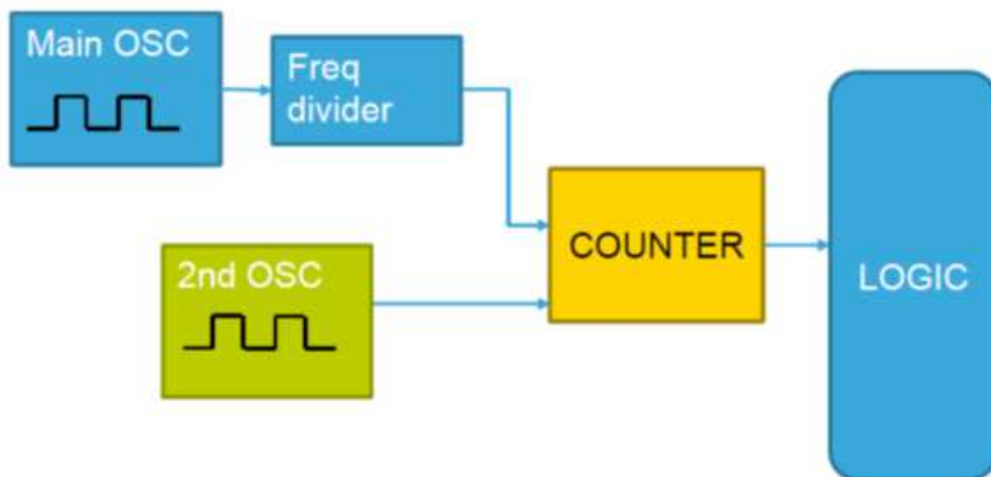
Figure 65. Oscillator monitor
