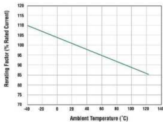
Figure 3: MAXI Temperature Derating Curve
