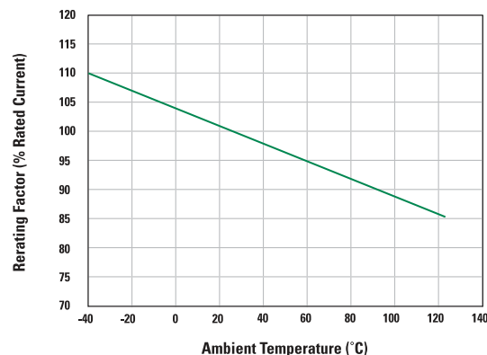
Figure 5: MINI Auto Fuse 297 Series Temperature Rerating Curve
