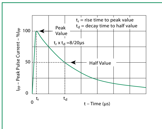
Figure 8 - Pulse Waveform
