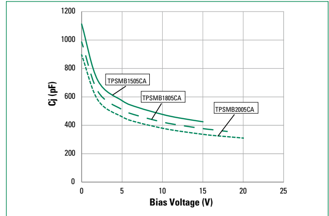
Figure 8 - Typical Junction Capacitance @TPSMBxx05CA(K to A)
