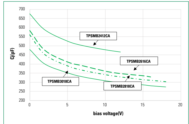
Figure 10 - Typical Junction Capacitance @ TPSMB2412/2616/2818CA(A to K)
