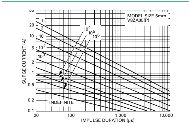
Figure 13 - V8ZA05P - V12ZA05P
