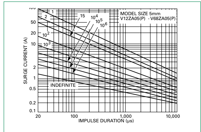
Figure 14 - V18ZA05(P) - V68ZA05(P)
