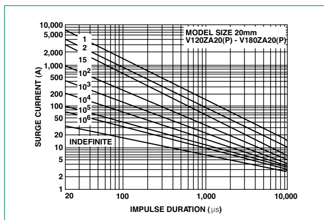
Figure 24 - V82ZA20(P) - V180ZA20(P)
