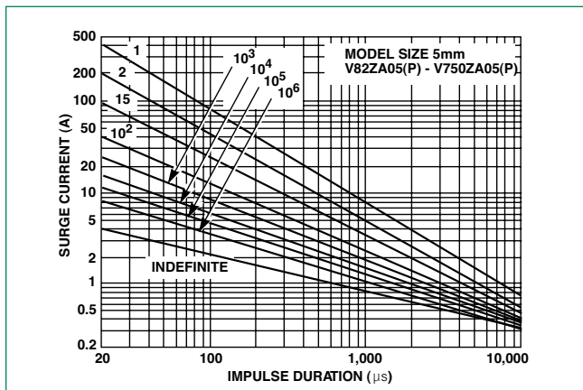
Figure 15 - V82ZA05(P) - V750ZA05(P)
