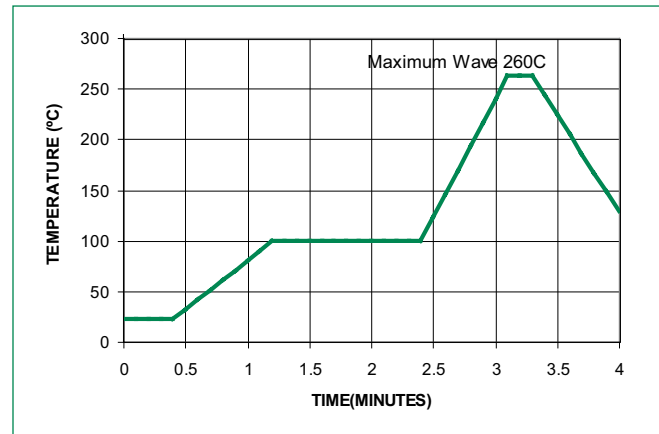
Figure 26 - Lead-free Profile
