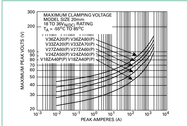
Figure 11 - V18ZA20(P) - V36ZA80(P)
