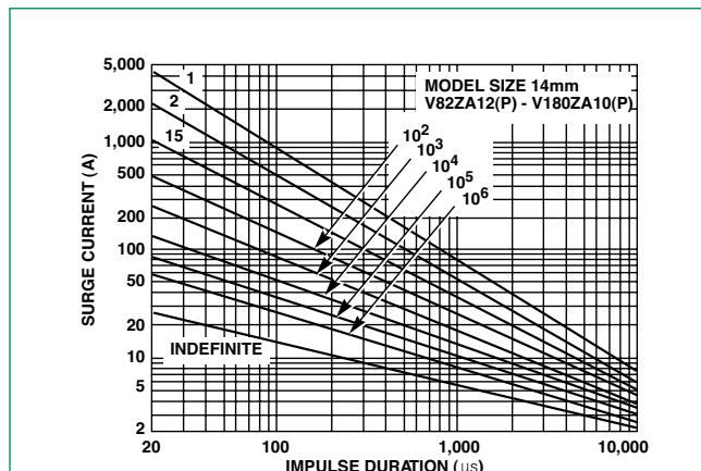
Figure 22 - V82ZA12(P) - V180ZA10(P)
