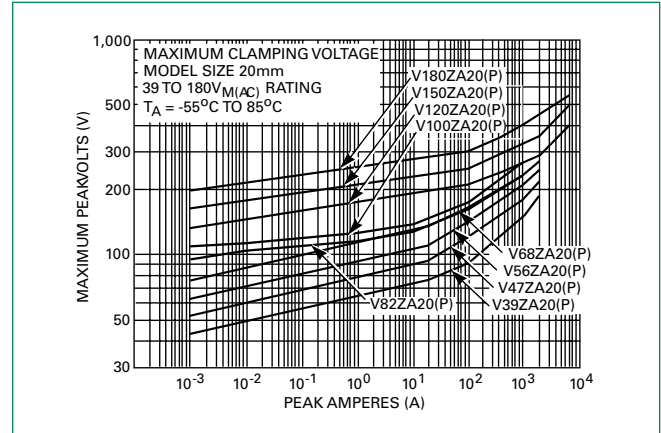
Figure 12 - V39ZA20(P) - V180ZA20(P)
