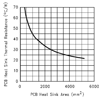
Figure 7-14. Heat Sink Thermal Resistance vs Area
