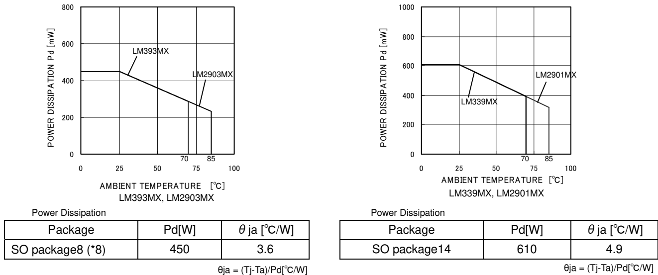
Fig.102 Derating Curves
