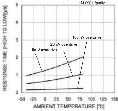
Fig. 86 Response Time (High to Low) – Ambient Temperature
