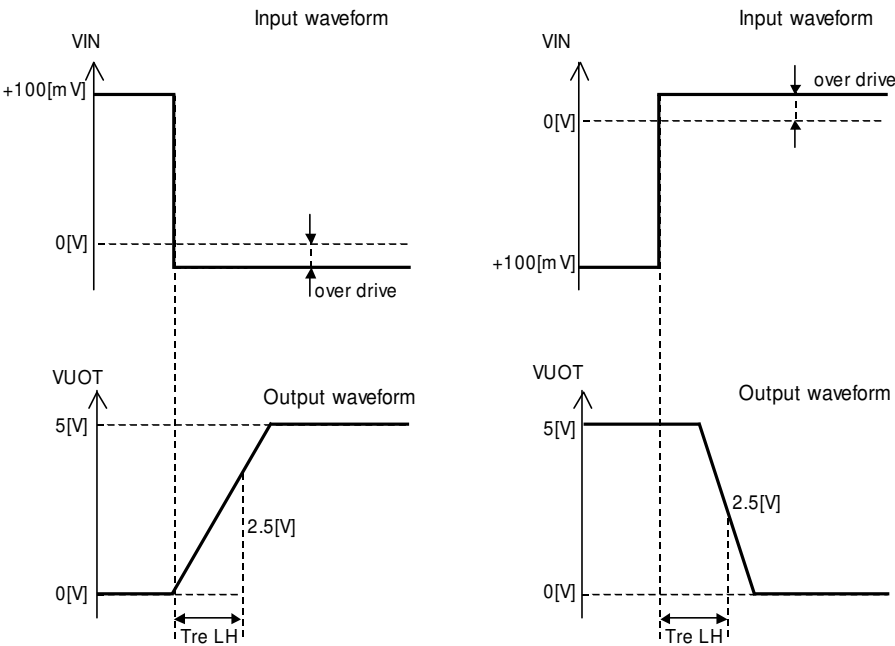
Fig.90 Response Time
