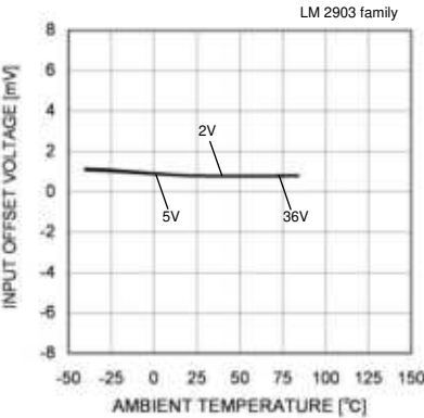
Fig. 49 Input Offset Voltage – Ambient Temperature
