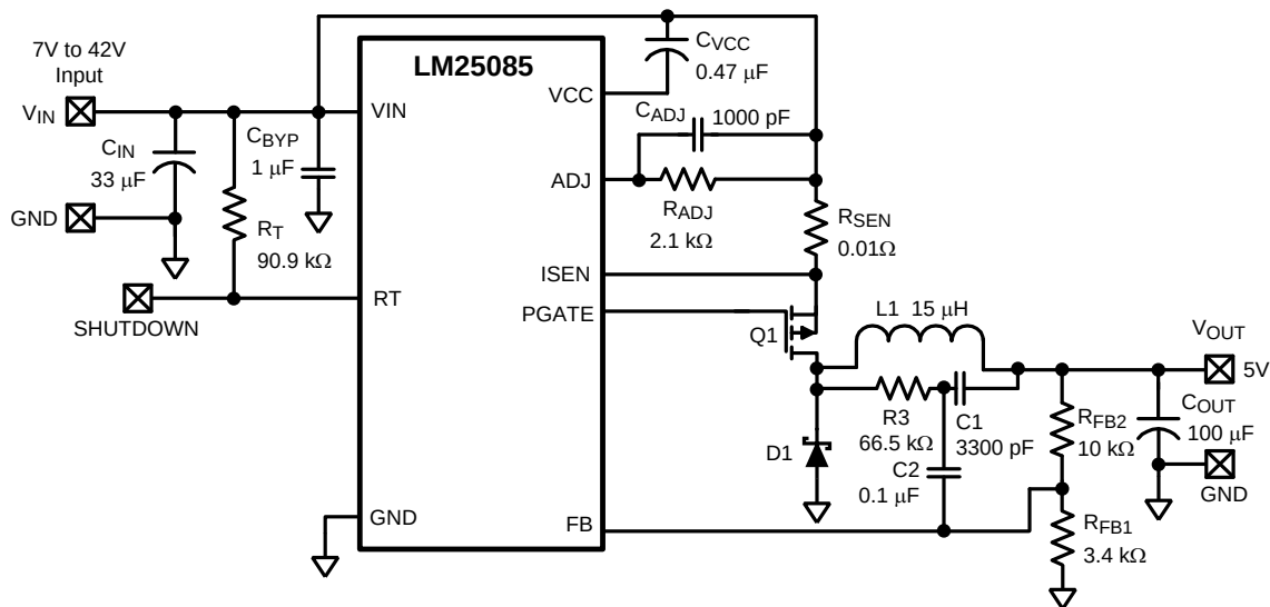
Figure 24. LM25085 Typical Application
