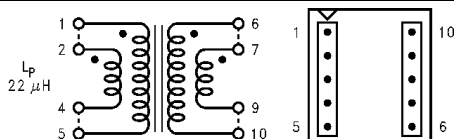
Figure 42. Schott 67141450 (Top View)
