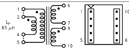
Figure 44. Schott 67140920 (Top View)
