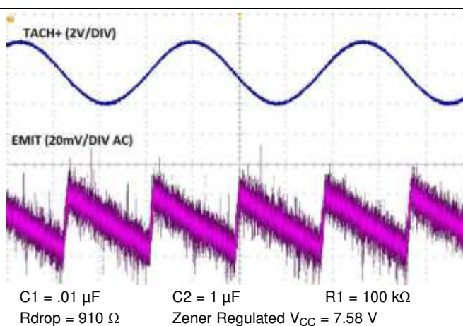
Figure 17. Output Voltage Ripple
