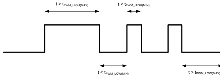
Figure 36. Simple Enable/Disable Timing
