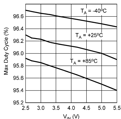
Figure 9. Max Duty Cycle vs V_{IN}
