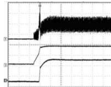
Channel 1: I_{IN} (200mA/div) Channel 3: V_{OUT} (20V/div) Channel 4 (10mA/div) L = 22\text{ }\mu\text{H} V_{IN} = 3.6\text{ V} Time Base (2ms/div) Ramp Rate = 8\mu\text{s/Step} I_{LED} = 19\text{ mA}
