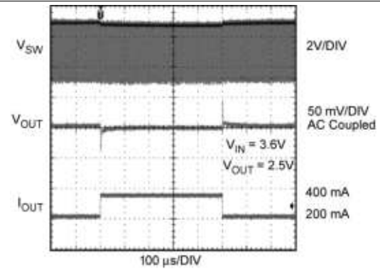
Figure 20. Load Transient Response (PWM Mode)
