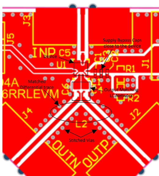
Figure 23. Supply Bypass and Output Matching
