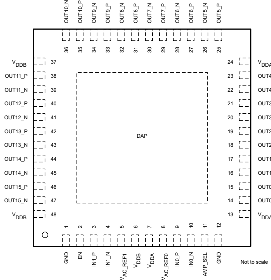
Figure 5-2. LMK1D2108: RGZ Package 48-Pin VQFN Top View
