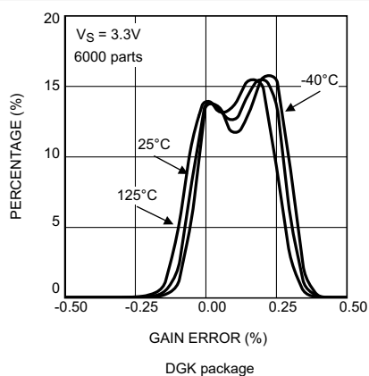
Figure 5-46. Gain Error Distribution at V_S = 3.3V LMP8601
