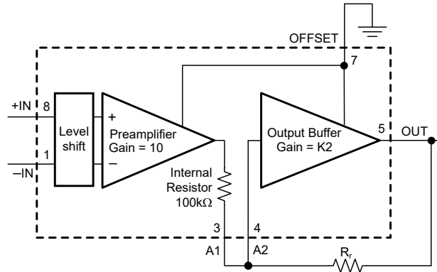
Figure 6-3. Increase Gain
