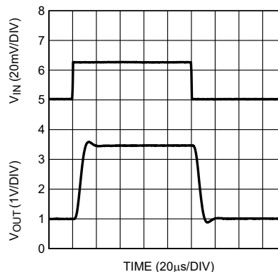
Figure 5-26. Step Response at V_S = 3.3V , R_L = 10k\Omega LMP8603
