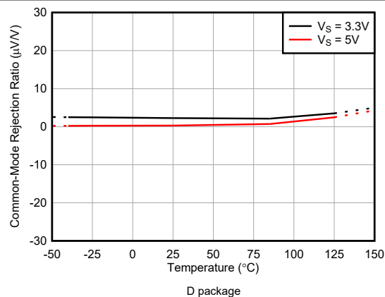
Figure 5-62. CMRR vs Temperature
