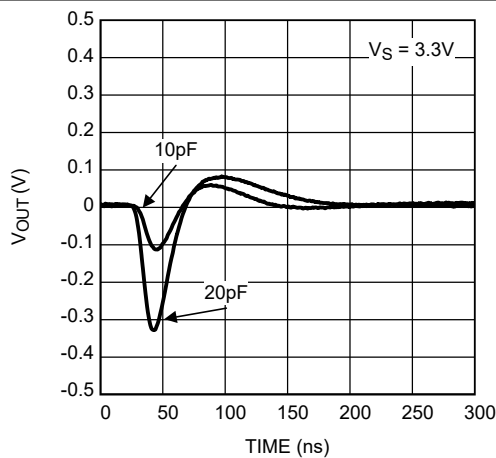
Figure 6-5. Capacitive Load Response at 3.3V
