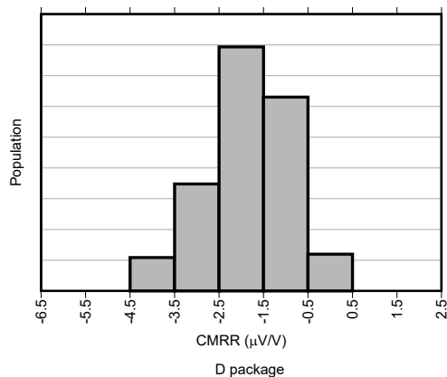
Figure 5-61. CMRR Distribution at V_S = 5V
