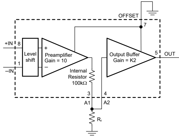
Figure 6-2. Reduce Gain
