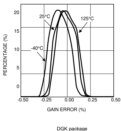
Figure 5-52. Gain Error Distribution at V_S = 5V , 5000 Parts LMP8602
