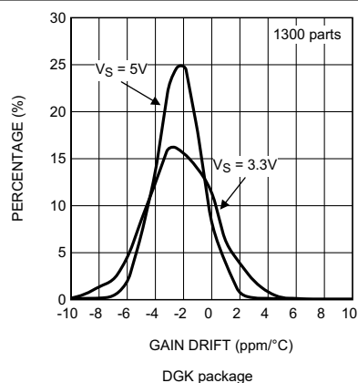
Figure 5-42. Gain Drift Distribution, 1300 Parts LMP8601
