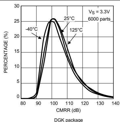
Figure 5-58. CMRR Distribution at V_S = 3.3V
