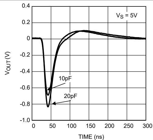
Figure 6-6. Capacitive Load Response at 5.0V
