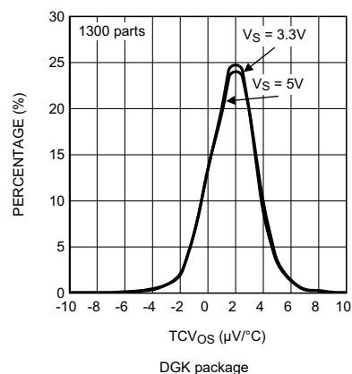
Figure 5-40. TCV_{OS} Distribution
