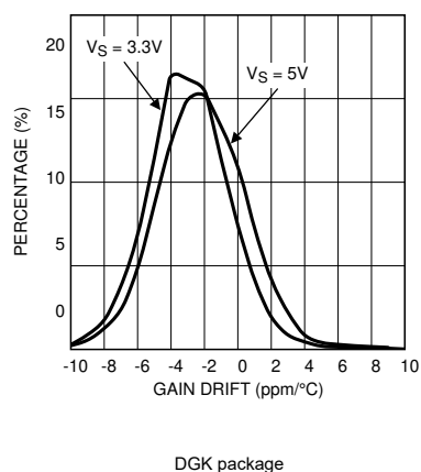
Figure 5-45. Gain Drift Distribution, 5000 Parts LMP8603
