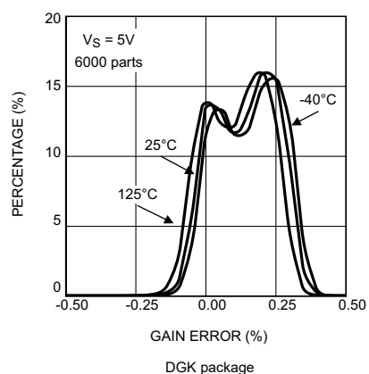
Figure 5-48. Gain Error Distribution at V_S = 5V LMP8601
