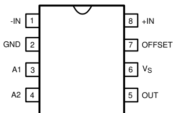
Figure 4-1. D Package 8-Pin SOIC Top View
