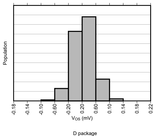
Figure 5-37. V_{OS} Distribution at V_S = 3.3V
