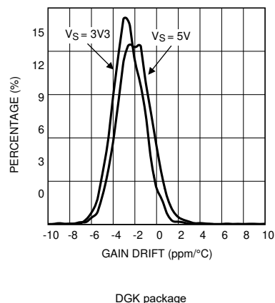
Figure 5-44. Gain Drift Distribution, 5000 Parts LMP8602
