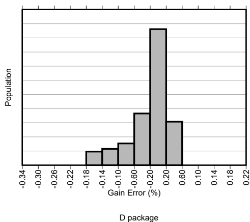
Figure 5-47. Gain Error Distribution at V_S = 3.3V LMP8601
