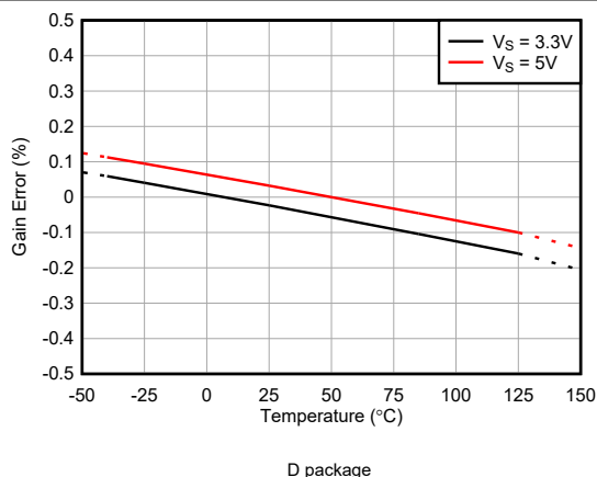
Figure 5-43. Gain Error vs Temperature for All Gains
