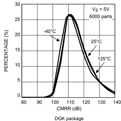
Figure 5-60. CMRR Distribution at V_S = 5V
