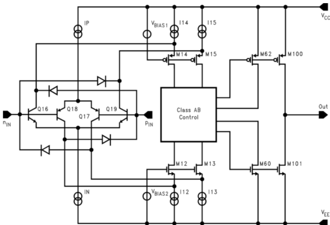
Figure 28. Simplified Schematic Diagram
