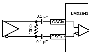
Figure 35. Differential Operation
