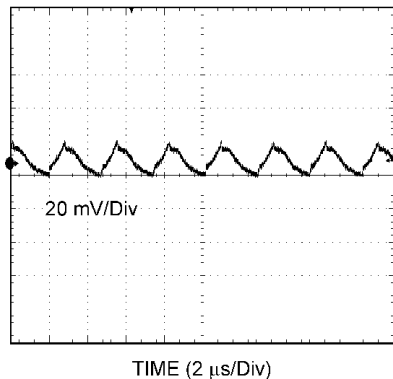
Figure 6-33. Output Ripple
