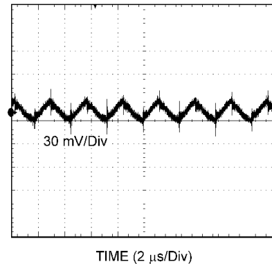
Figure 6-34. Output Ripple
