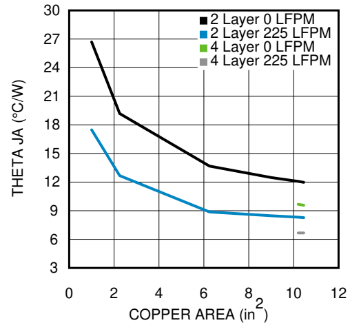
Figure 6-32. R_{\theta JA} vs Copper Heat Sinking Area
