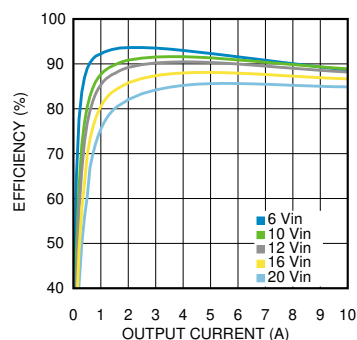
Efficiency 3.3-V Output at 25^{\circ}\text{C}
