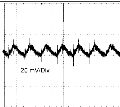
Figure 34. Output Ripple
