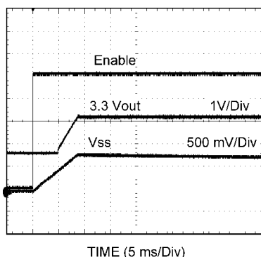
Figure 45. Prebiased Start-Up
