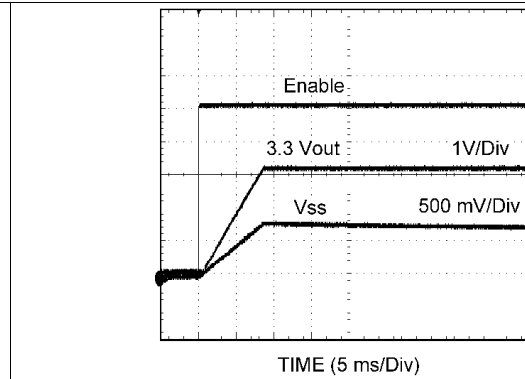
Figure 44. 3.3 V OUT Soft-Start
