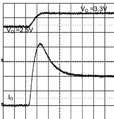
Figure 23. Prebiased Start-Up
