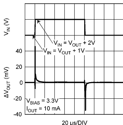
Figure 24. V_{IN} Line Transient Response
