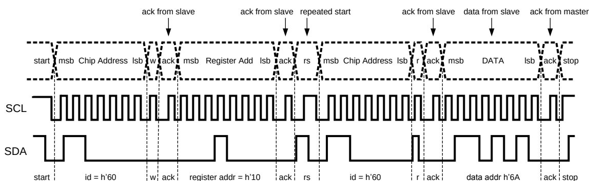
Figure 63. I 2 C Read Cycle
