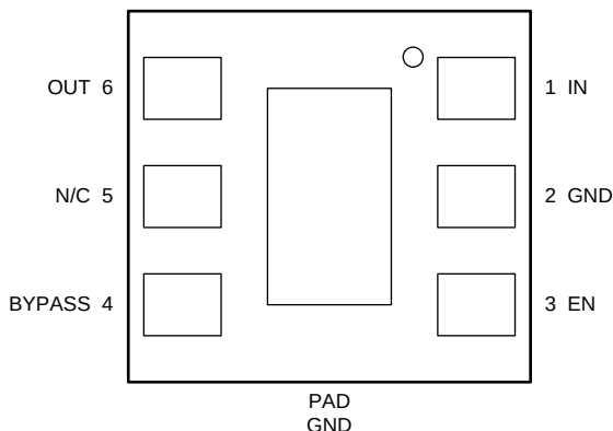
NGD Package 6-Pin WSON Top View
