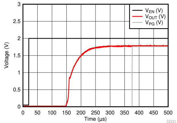
Figure 6-38. LP5912-1.8 V_{OUT} vs V_{EN(ON)}
