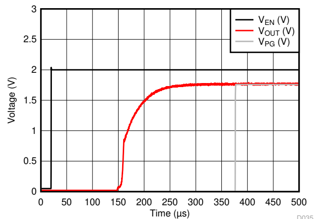
Figure 6-40. LP5912-1.8 V_{OUT} vs V_{EN(ON)}
