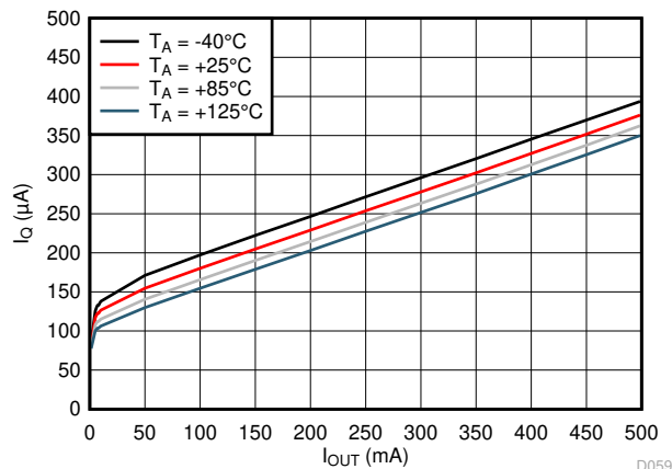
Figure 6-19. LP5912-3.3 I_{Q(SD)} vs I_{OUT}
