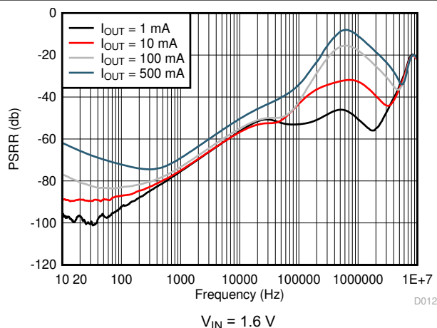
Figure 6-21. LP5912-0.9 PSRR vs Frequency
