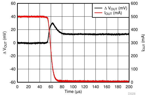
Figure 6-37. LP5912-3.3 Load Transient Response
