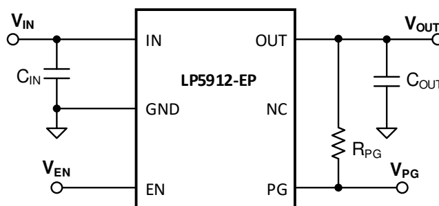
Simplified Schematic
