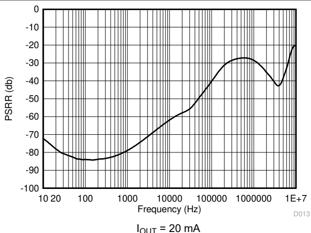
Figure 6-22. LP5912-1.8 PSRR vs Frequency
