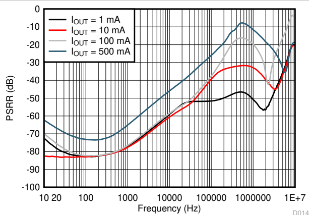
Figure 6-21. LP5912-0.9 PSRR vs Frequency
