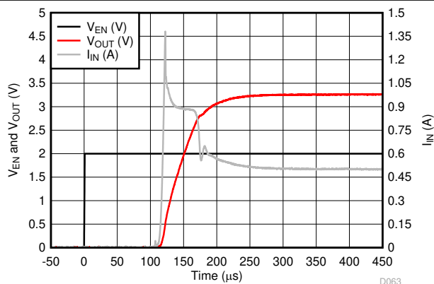
Figure 6-52. LP5912-3.3 Inrush Current
