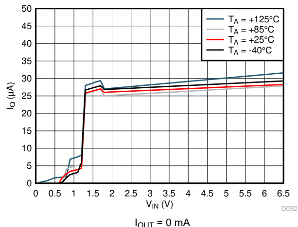
Figure 6-12. LP5912-1.8 I_Q (No Load) vs V_{IN}
