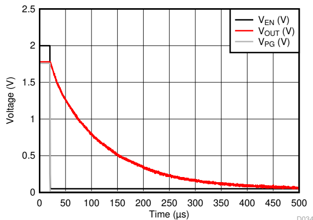
Figure 6-39. LP5912-1.8 V_{OUT} vs V_{EN(OFF)}
