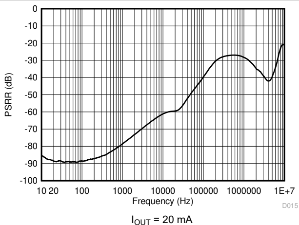
Figure 6-24. LP5912-3.3 PSRR vs Frequency
