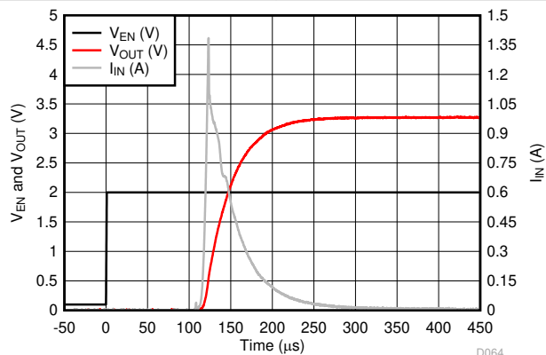
Figure 6-51. LP5912-3.3 Inrush Current
