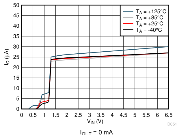
Figure 6-11. LP5912-0.9 I_Q (No Load) vs V_{IN}
