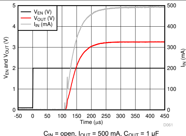
Figure 6-50. LP5912-3.3 Inrush Current
