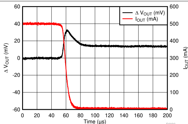
Figure 6-33. LP5912-0.9 Load Transient Response
