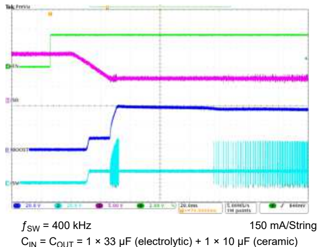
Figure 8-4. Typical Start-Up
