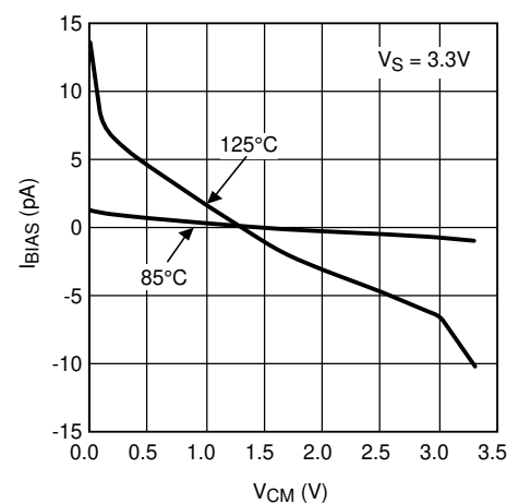
Figure 5-36. Input Bias Current vs Common Mode Voltage
