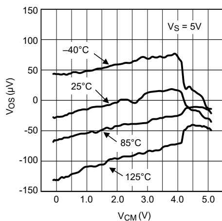
Figure 5-11. Input Offset Voltage vs Input Common Mode
