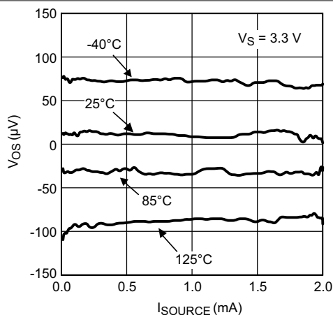
Figure 5-18. Input Offset Voltage vs Sourcing Current
