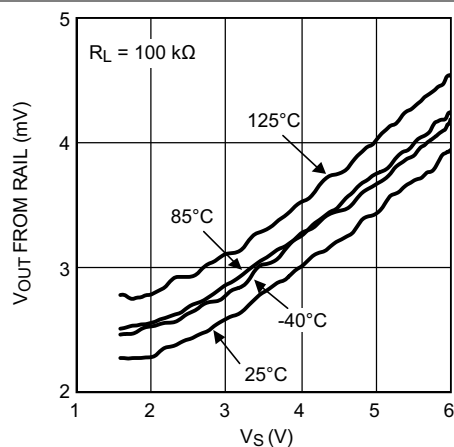
Figure 5-32. Output Swing Low vs Supply Voltage
