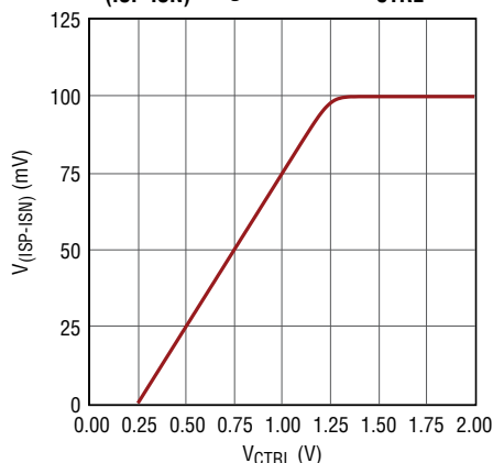
V_{(ISP-ISN)} Regulation vs V_{CTRL}
