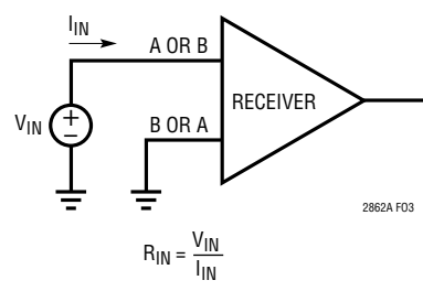
Figure 3. Receiver Input Current and Input Resistance
