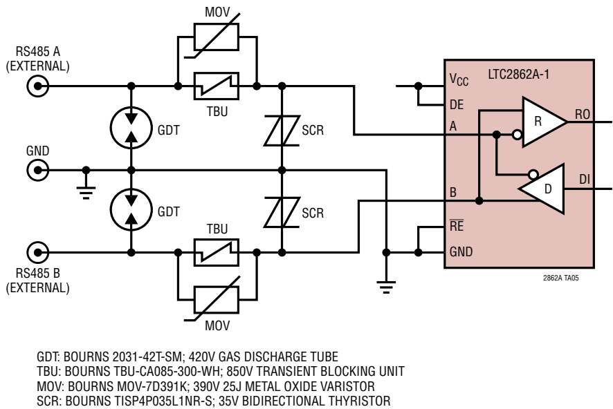
Network for IEC Level 4 Protection Against 5kV Surge, 5kV EFT and 30kV IEC ESD Plus ±360V Overvoltage Protection
