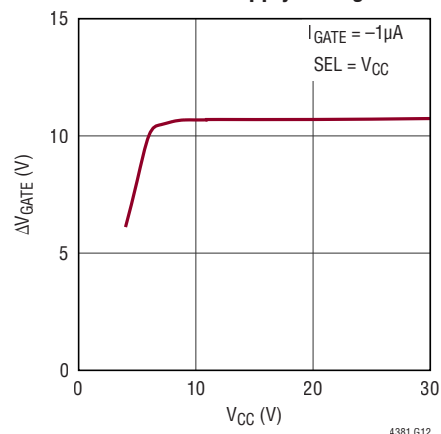
Gate Drive vs Supply Voltage
