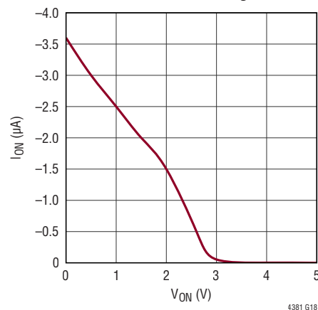
ON Pin Current vs Voltage
