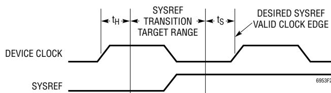
Figure 23. SYSREF Edge Timing Example
