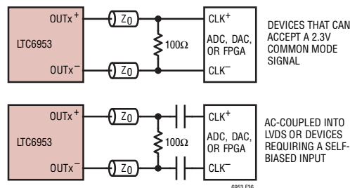
Figure 36. OUTx CML Connections to Device Clock Inputs ( Z_0 = 50\Omega )
