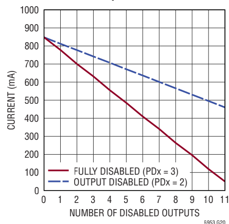
Supply Current vs Number of Disabled Outputs
