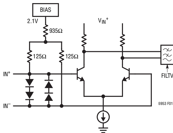
Figure 1. Simplified Input Interface Schematic
