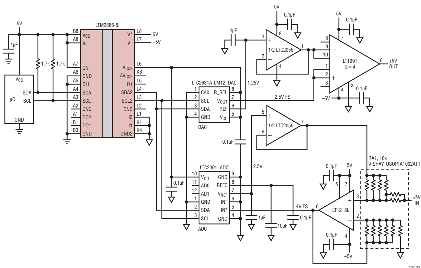
Figure 20. Isolated I 2 C 12-Bit, \pm 5V Analog Input and Output
