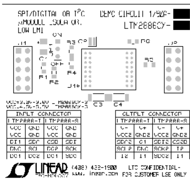
Figure 17. LTM2886 Low EMI Demo Board Layout
