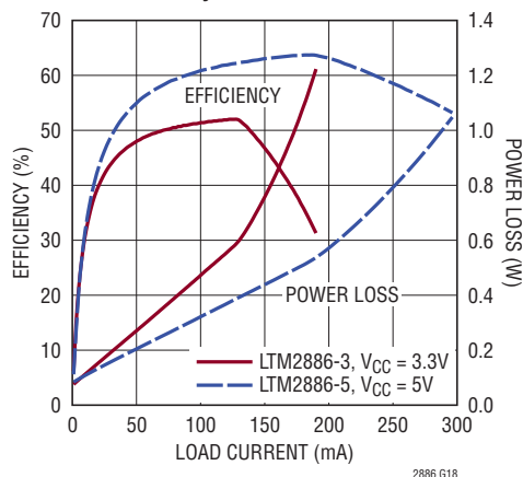
V^+ Efficiency
