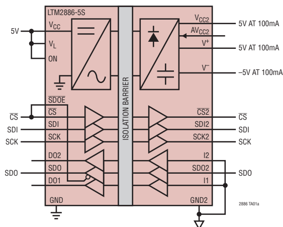
Isolated 4MHz SPI Interface
