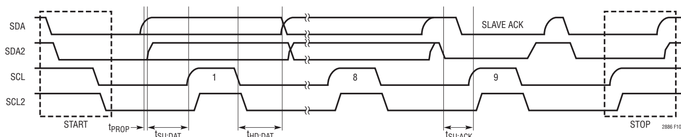
Figure 10. I²C Timing Diagram
