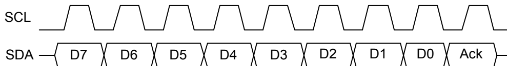
Signal pattern of the I 2 C byte write
