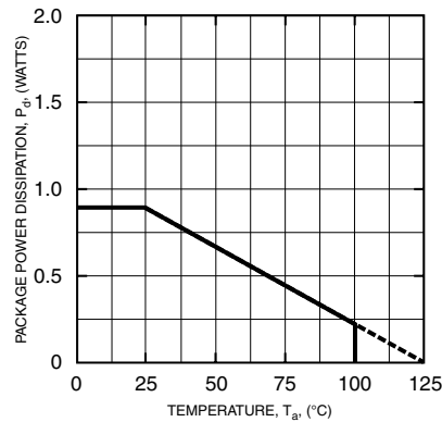
THERMAL DERATING CHARACTERISTICS
