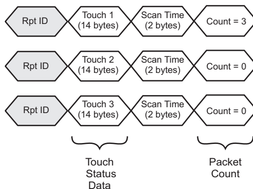
Figure 10-13. Example Touch Report Packets for 3 Active Touches
