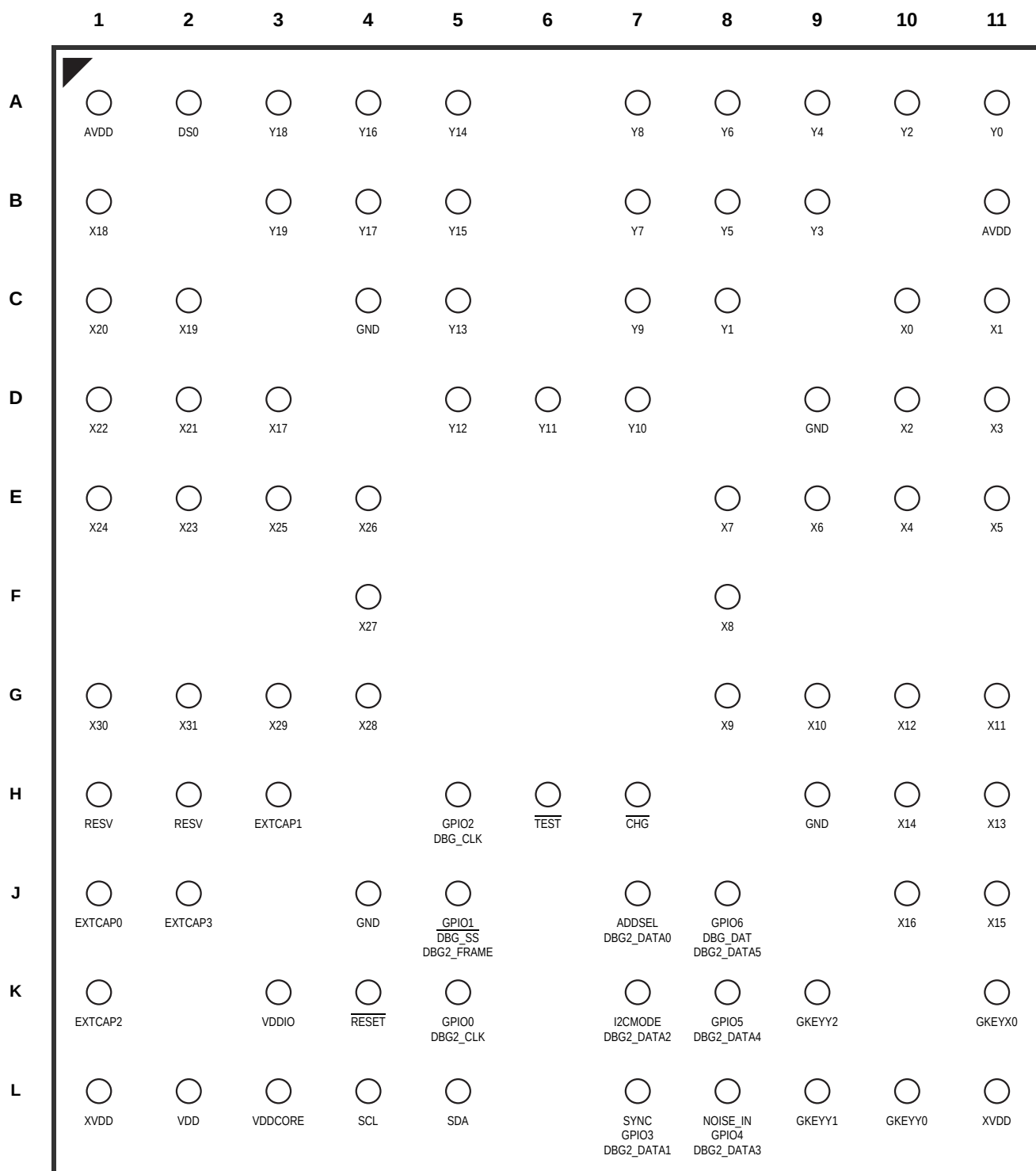
Top View
